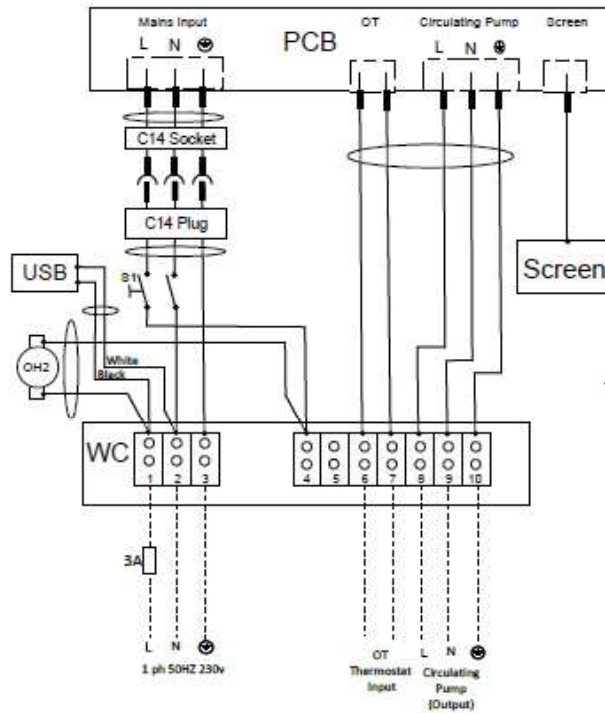
Internal Wiring Diagram (Sapphire PCB Connections)
